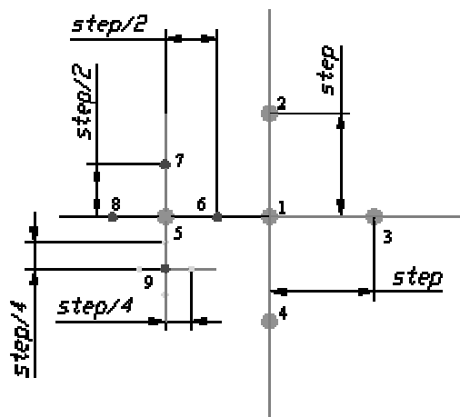
Fig. 4. The scheme of the approximating process
