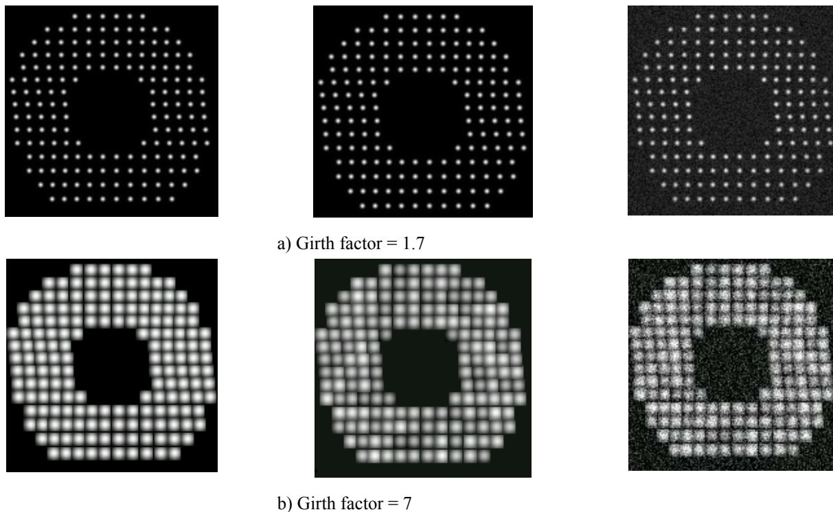
Fig. 5. A sequence of hartmanogramm creation with various values of girth factor.
