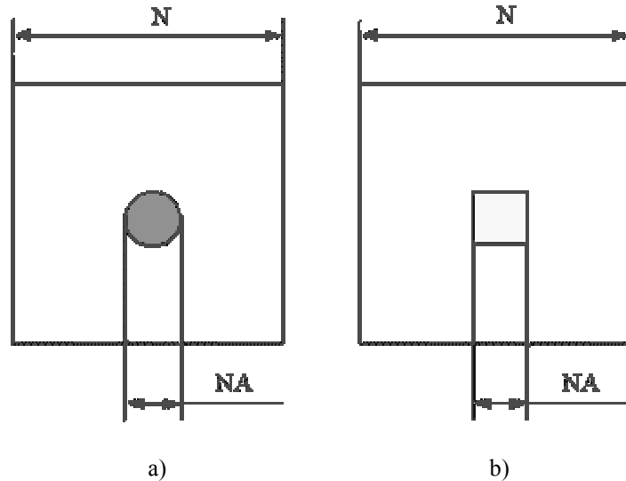
Fig. 3. The pupil function formation for approximation function reception of intensity dispersion in spot: a) - for the round aperture; b) - for the rectangular aperture.
